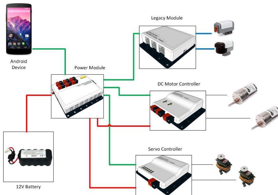
Figure 5 - K9 bot hardware with USB-enabled motor/servo controllers (cables and adapter not shown in detail).
