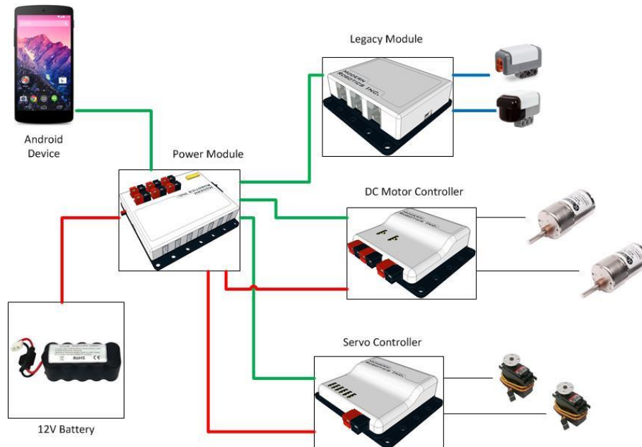
Figure 102 - This diagram shows how the devices are connected on the typical K9 bot.
