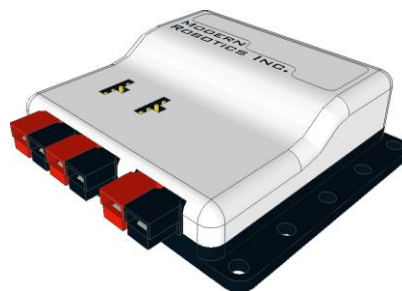
Figure 7 - New Motor Controller has two DC motor channels and uses Anderson Power Pole connectors
